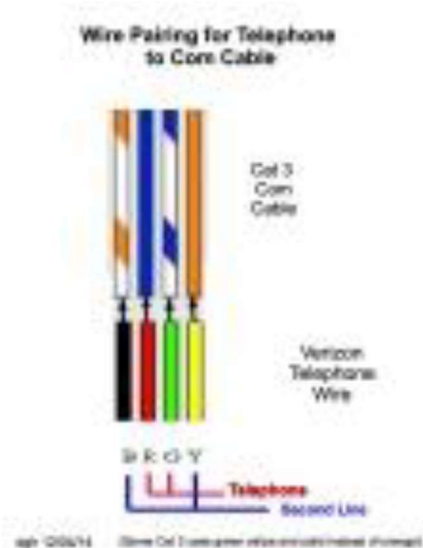
Telephone wire pairing
